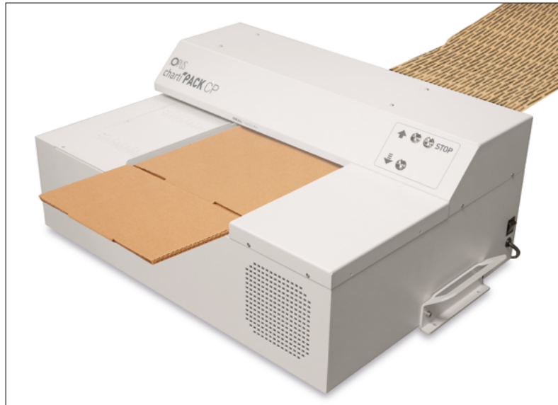
chartiPACK CP shredder in operation. Uncut cardboard is inserted into the feed slot. On the other side of the device is a slot from which the finished cut filler comes out.
